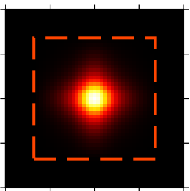
(50) Sech
