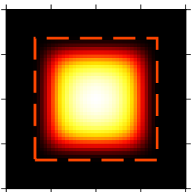
(47) Power law
