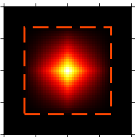
(48) Root
