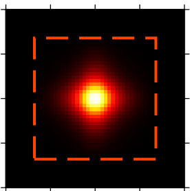
(49) Circular
