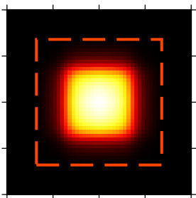
(46) Inverse multiquadric
