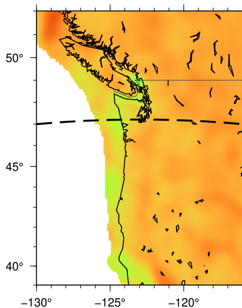
(e) Vs aggregate: z = 2 km
