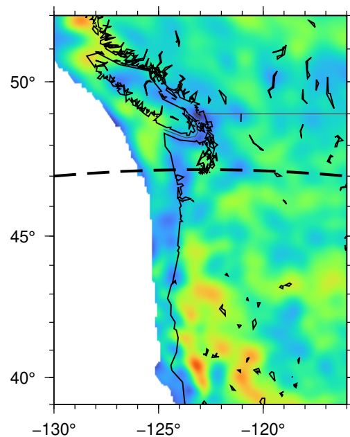
(f) Density aggregate: z = 2 km
