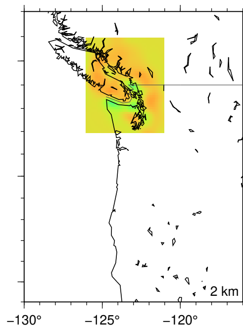
(e) Cascadia v1.6: Original
