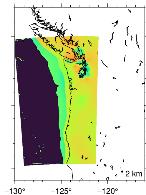
(e) Cascadia v1.6: Original
