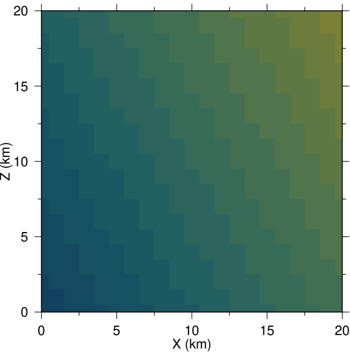
(c) Vs Original: y = 10 km
