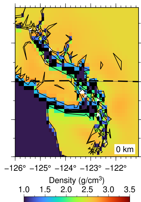
(f) Original Density
