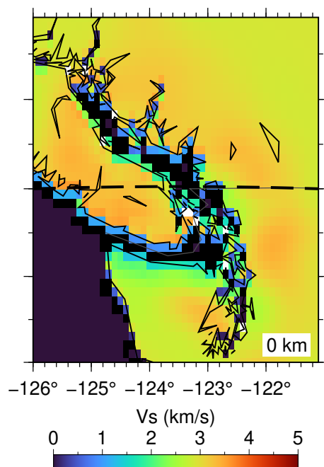
(e) Original Vs
