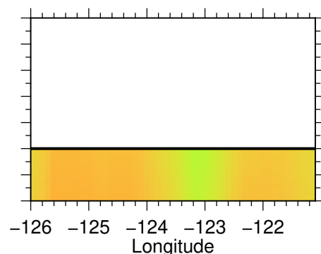
(i) Linear Density
