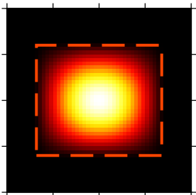
(36) Quintic
