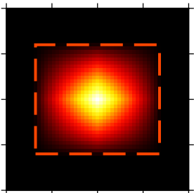
(37) Septic
