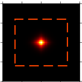
(42) Gompertz
