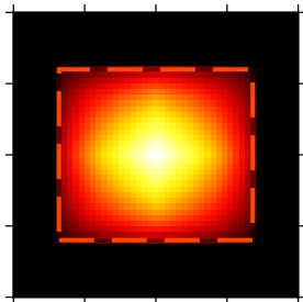
(52) Student
