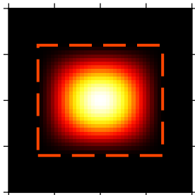
(38) Nonic
