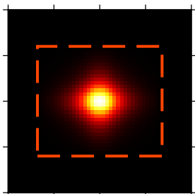
(49) Circular
