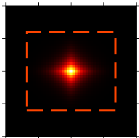
(53) Laplace
