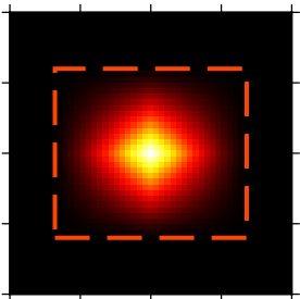
(51) Sech squared
