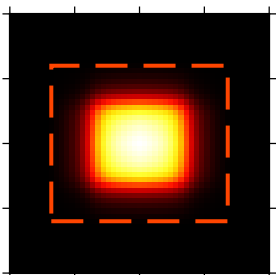
(46) Inverse multiquadric
