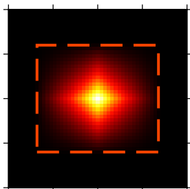
(48) Root
