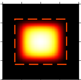
(47) Power law
