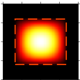
(35) Quartic
