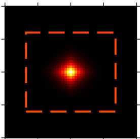
(41) Arctan
