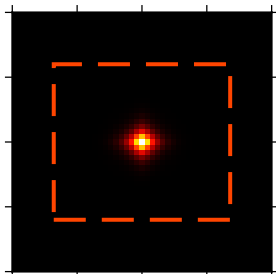
(43) Softsign
