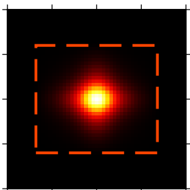
(50) Sech
