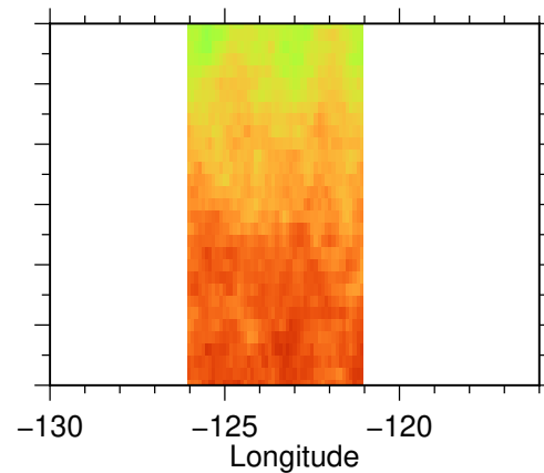
(c) SVI EQTOMO: Perturbed
