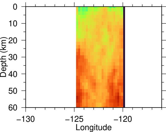
(a) Cascadia ANT+RF: Perturbed
