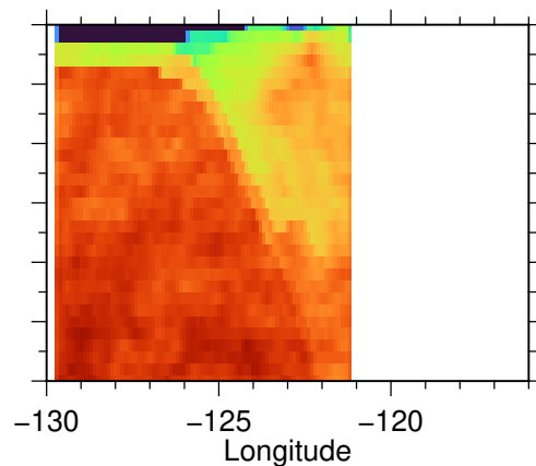
(e) Cascadia v1.6: Perturbed
