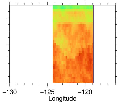
(b) PNW10-S: Perturbed
