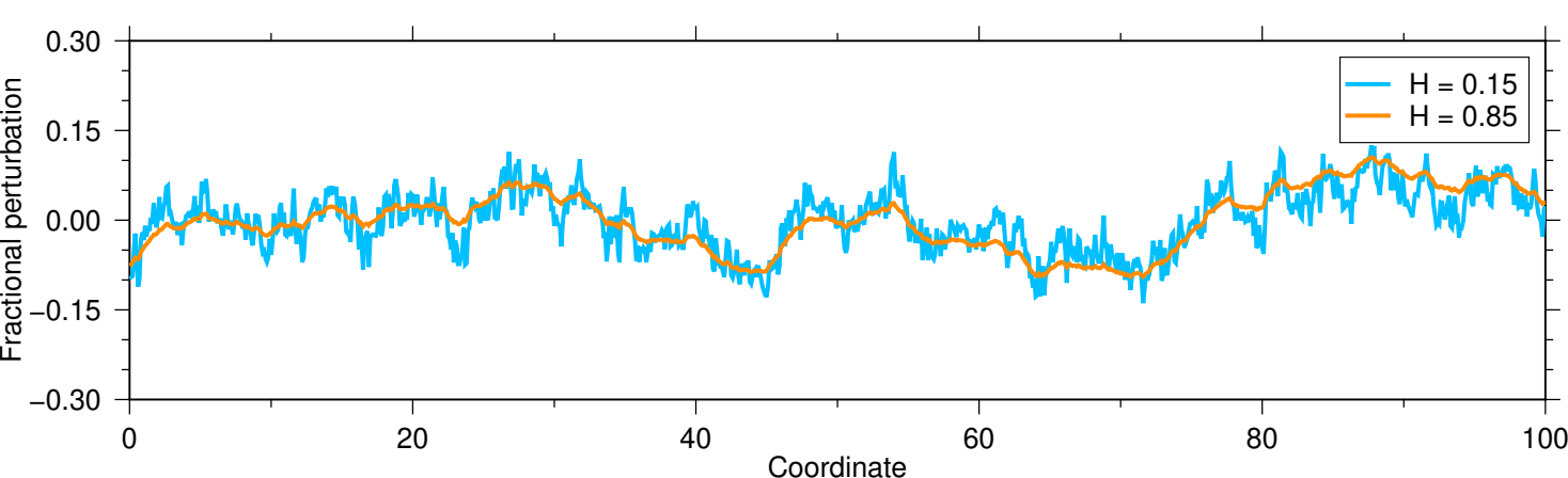
(c) Hurst exponent
