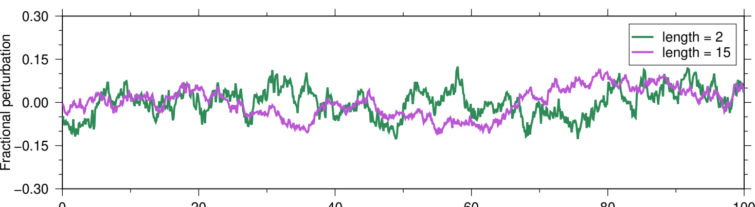
(c) Hurst exponent
