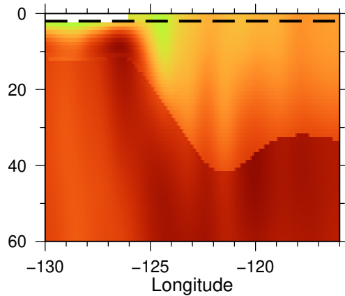
(e) Vs aggregate: latitude = 47 N
