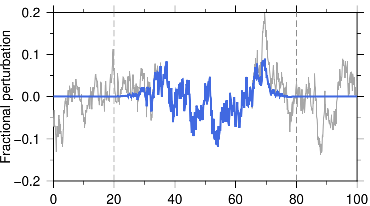
(e) Gaussian
