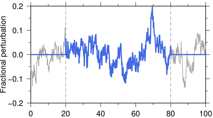
(c) Cosine
