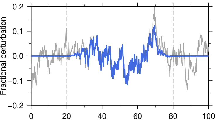
(e) Gaussian
