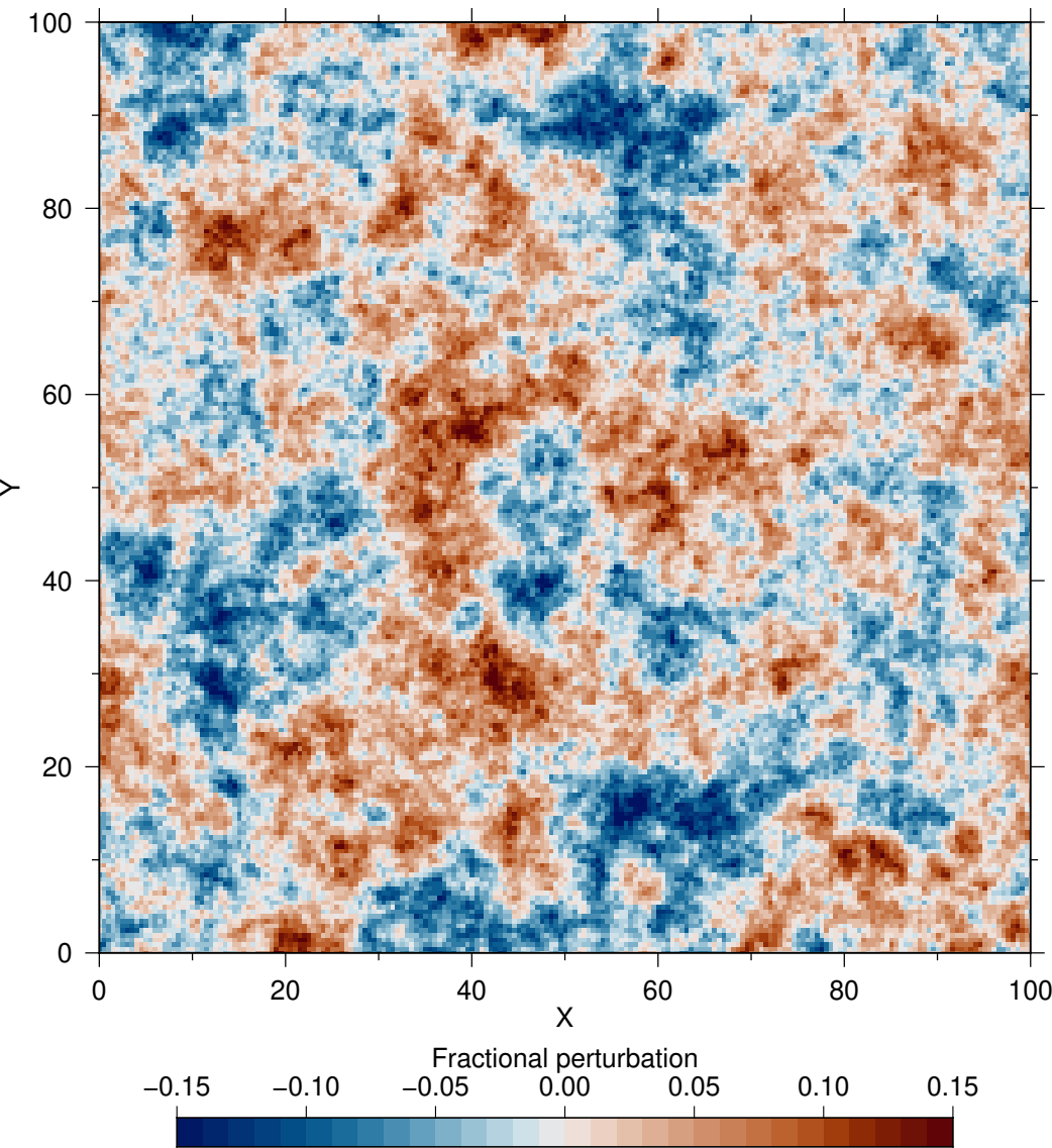
Two-dimensional von Karman heterogeneity
