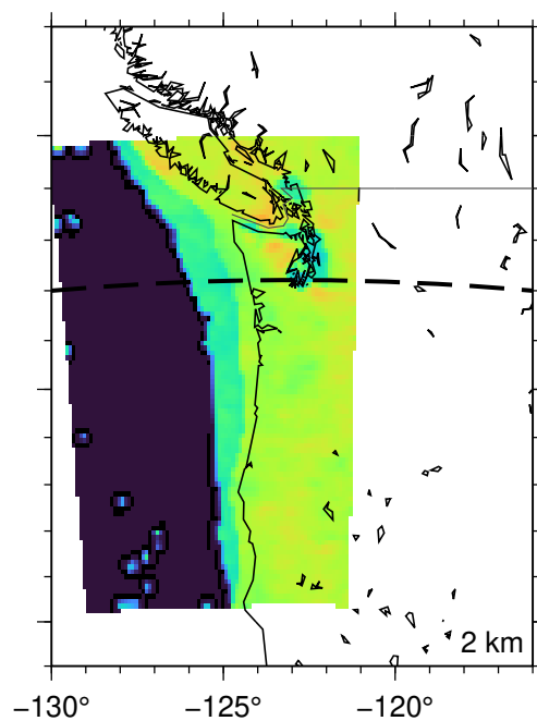
(e) Cascadia v1.6: Perturbed
