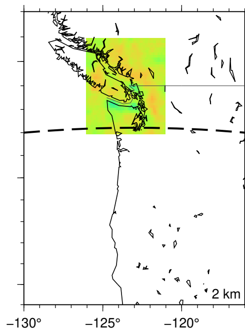
(e) Cascadia v1.6: Perturbed
