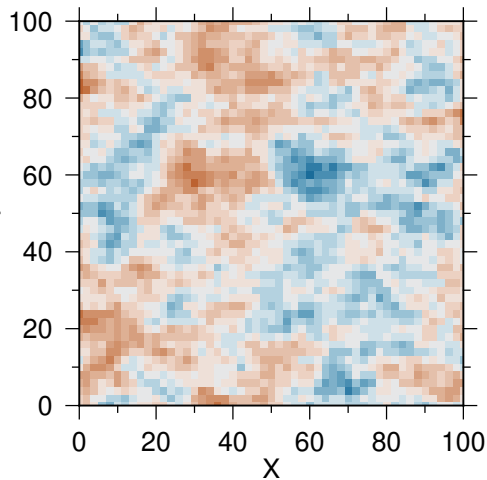
(a) Vp: sigma 2.5%
