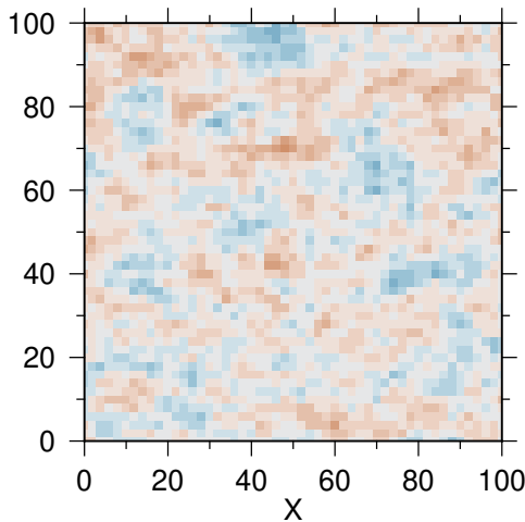
(c) Density: sigma 1.5%
