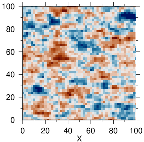
(b) Vs: sigma 5%
