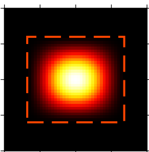
(7) Welch
