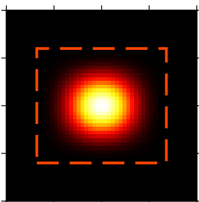
(19) Cubic
