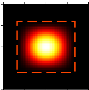
(15) Nuttall
