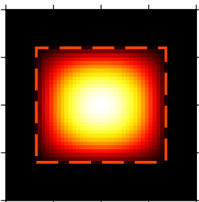
(12) Exponential
