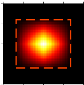
(25) Logistic
