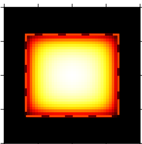
(17) Cauchy
