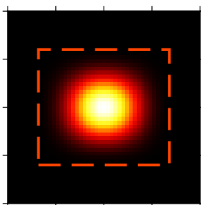
(10) Smoothstep
