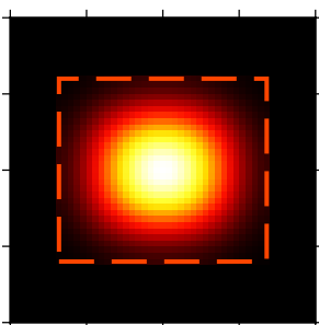
(9) Gaussian
