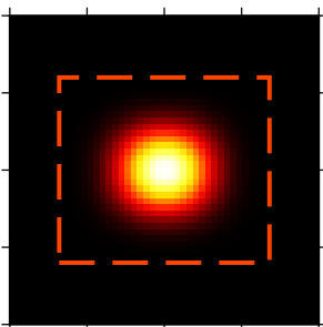
(11) Smotherstep
