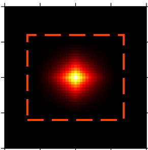
(24) Planck taper
