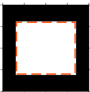
(6) Blackman-Harris
