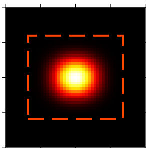
(20) Bartlett
