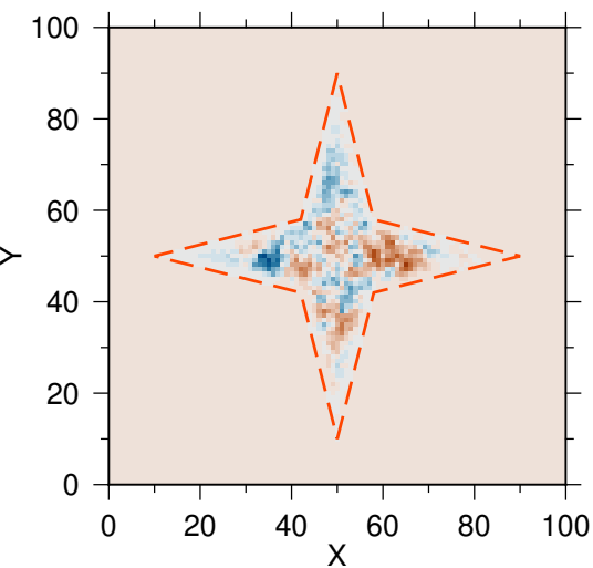
(e) Gaussian
