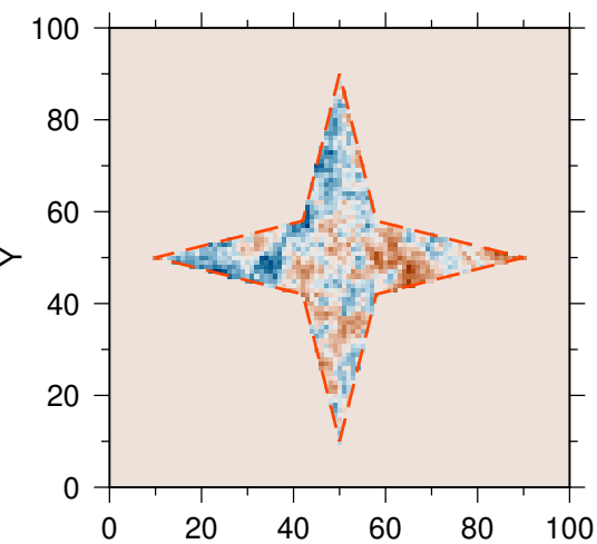
(a) Boxcar
