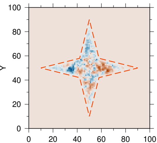
(c) Cosine
