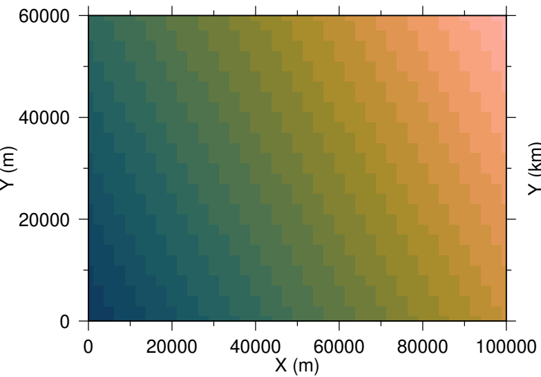
(a) Source: m and m/s
