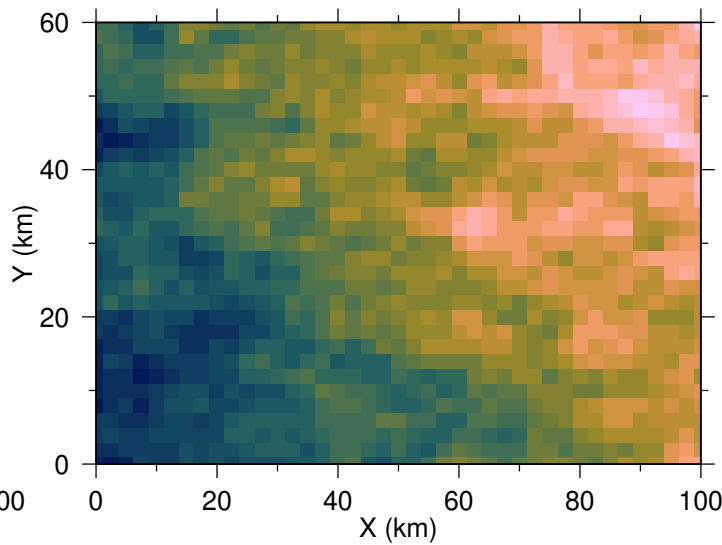
(b) Scaled and perturbed
