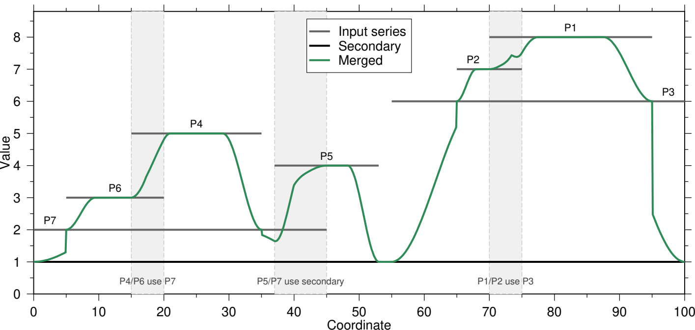
(b) With aggregate mode (-A)
